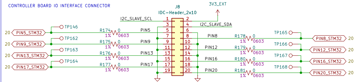
CONTROLLER BOARD IO INTERFACE CONNECTOR
