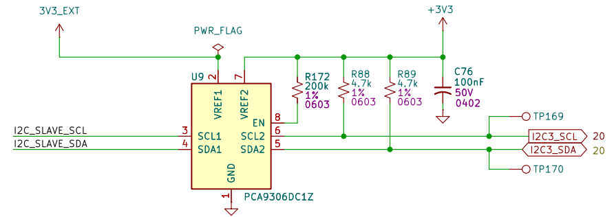
I2C BUFFER
